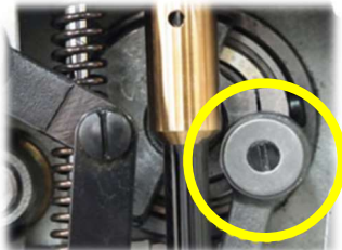
Easy needle stroke change (31mm ⇄ 33mm) with a minus screw driver
