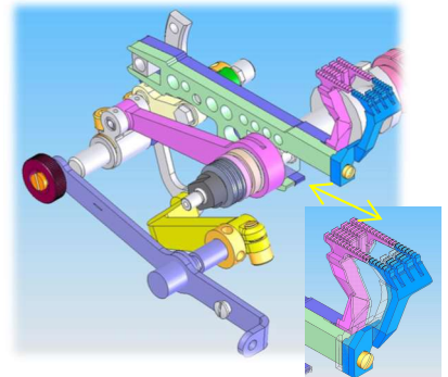
Angle adjustable rear feed dog for difficult materials
